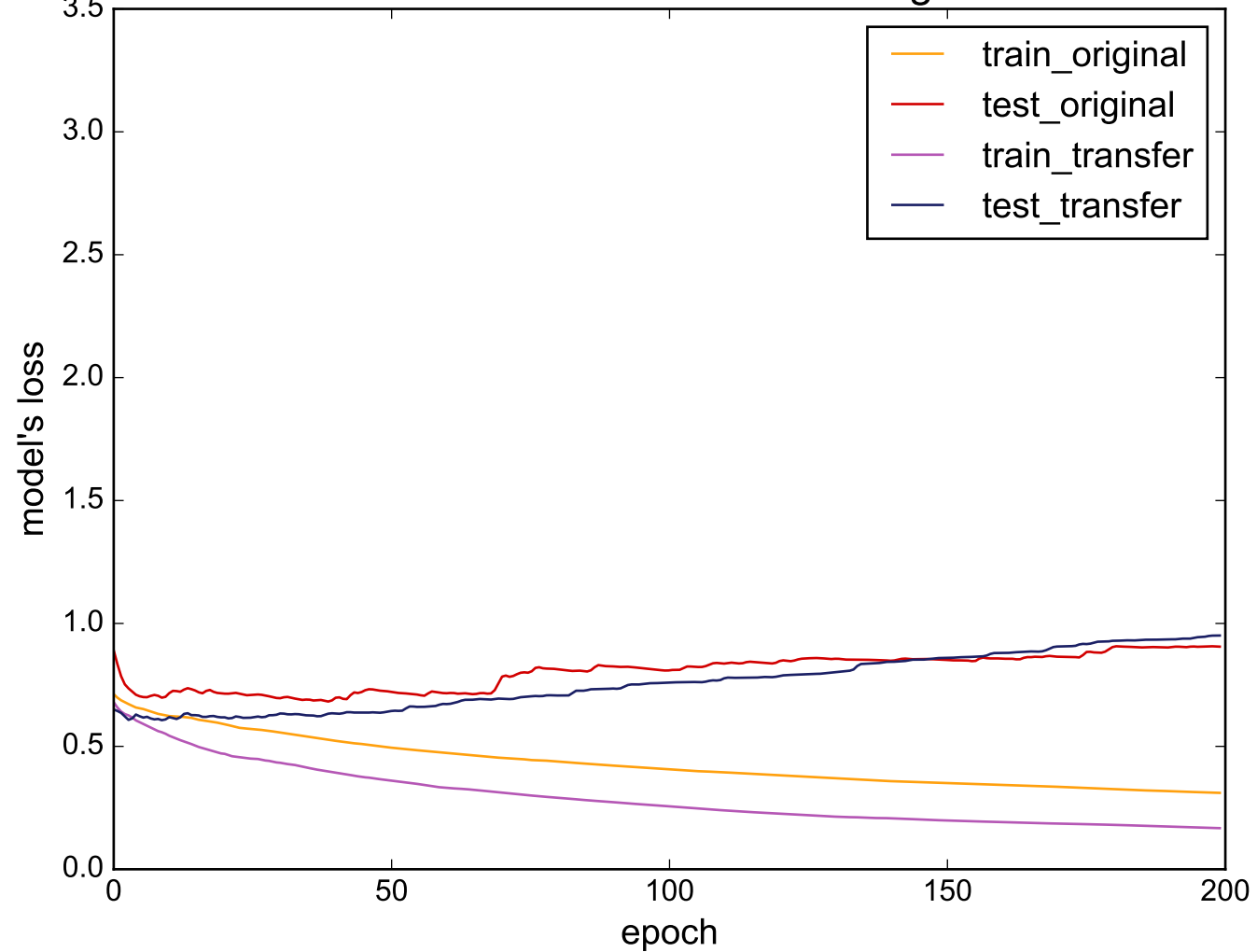
Source: ProximalPhalanxTW - Target: Ham
