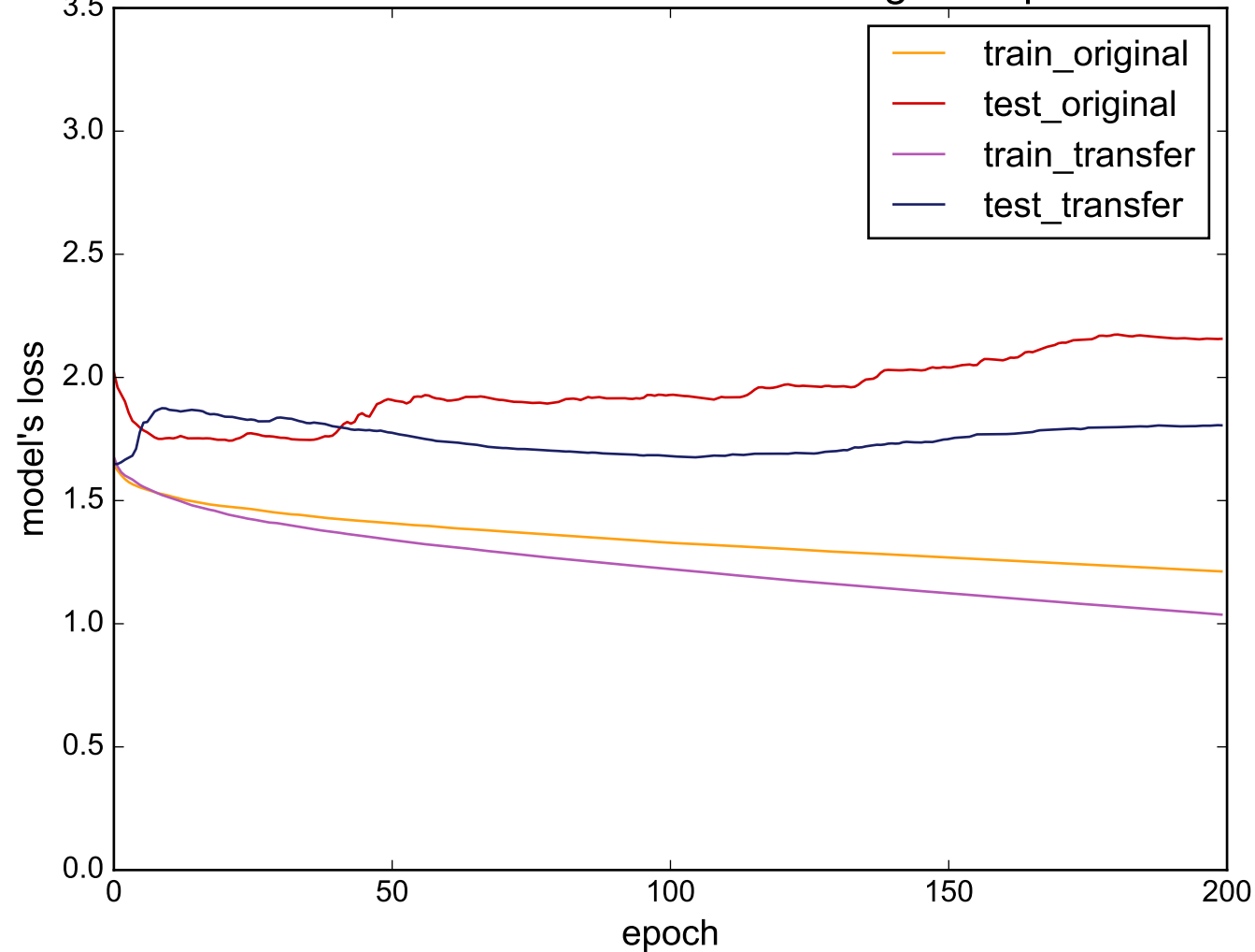
Source: ProximalPhalanxTW - Target: Haptics
