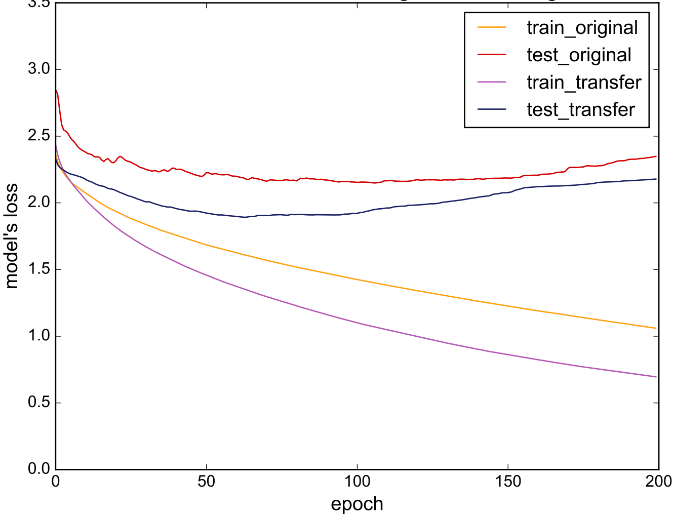
Source: ProximalPhalanxTW - Target: InsectWingbeatSound
