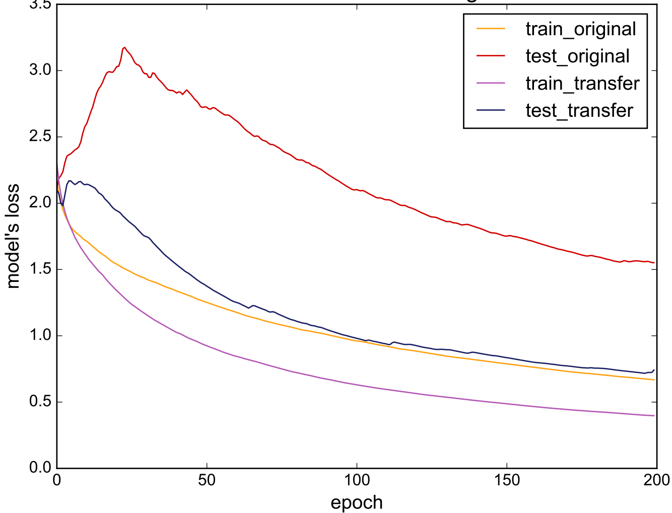
Source: ProximalPhalanxTW - Target: MALLAT
