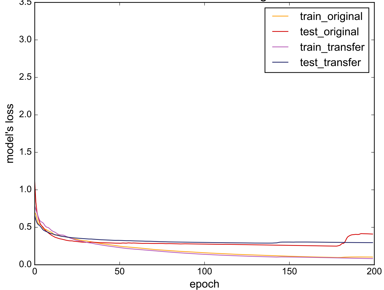
Source: ProximalPhalanxTW - Target: MoteStrain
