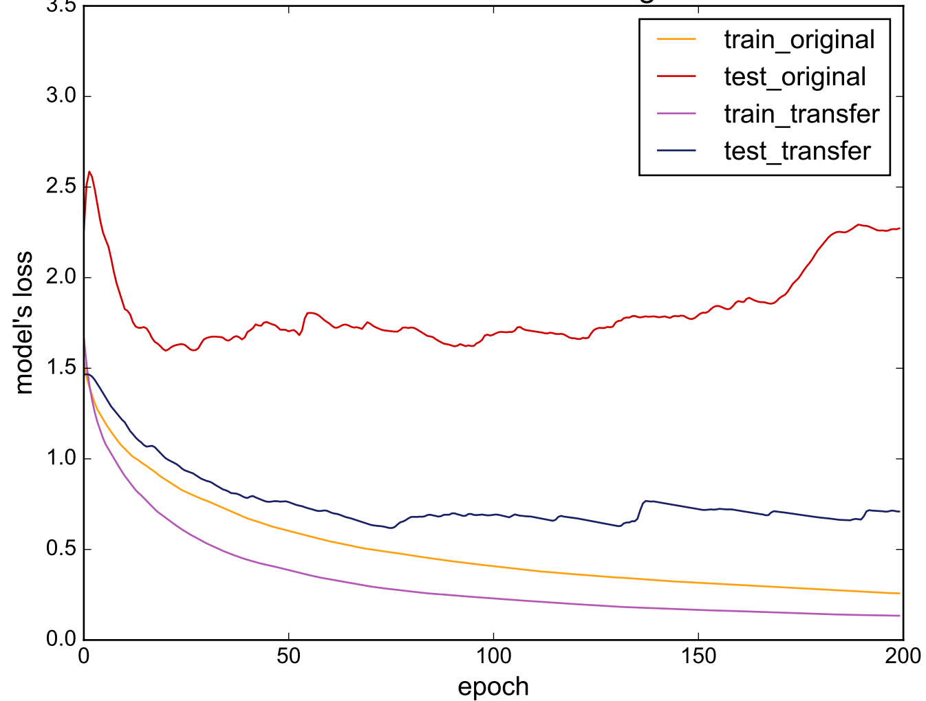
Source: ProximalPhalanxTW - Target: OSULeaf
