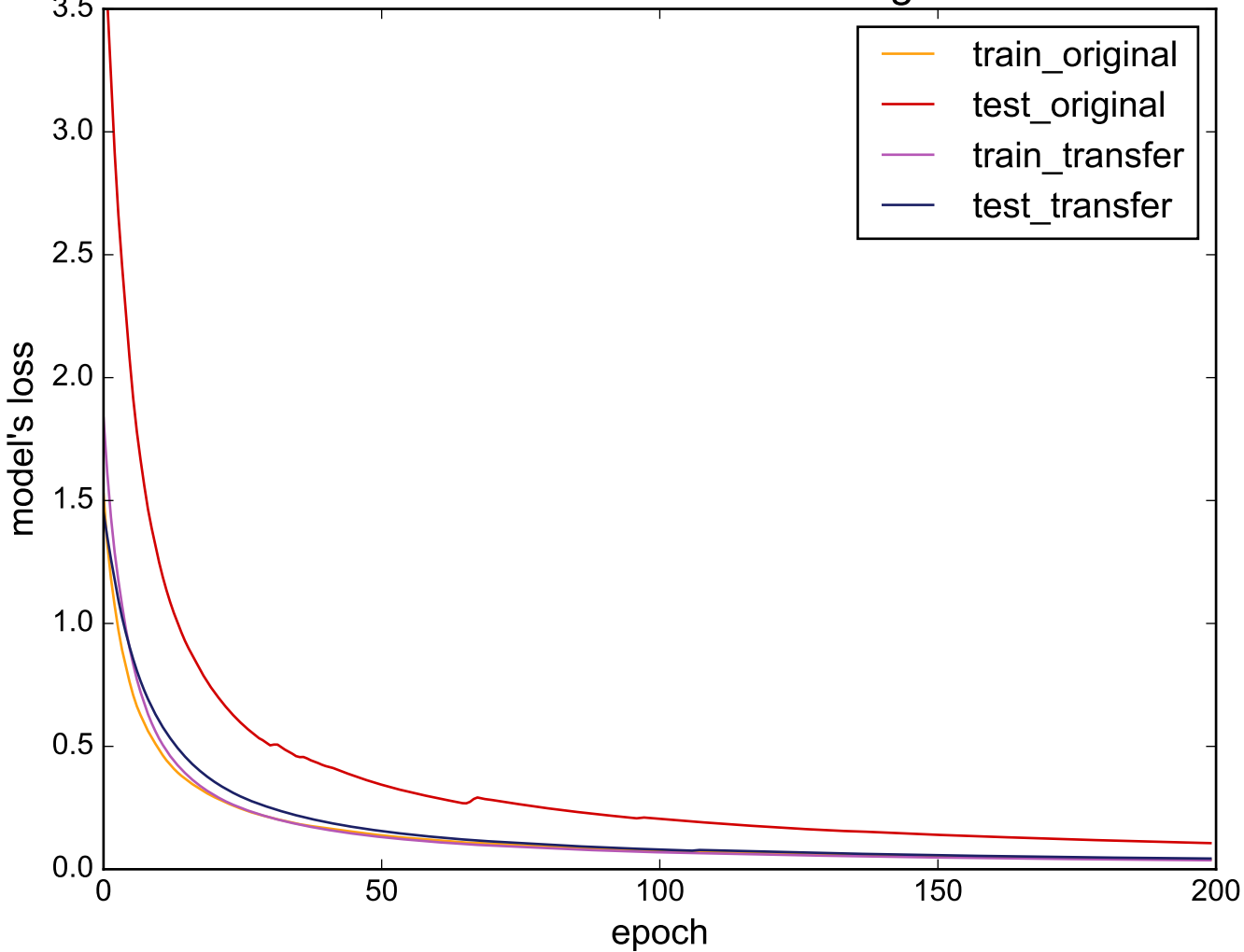
Source: ProximalPhalanxTW - Target: Plane
