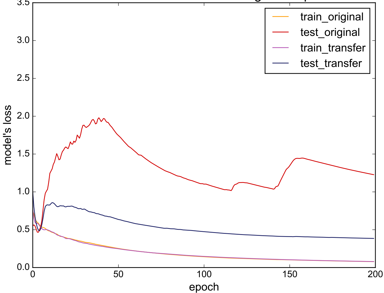
Source: ProximalPhalanxTW - Target: ShapeletSim
