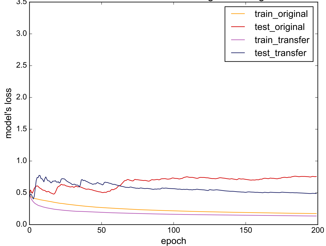
Source: ProximalPhalanxTW - Target: StarLightCurves
