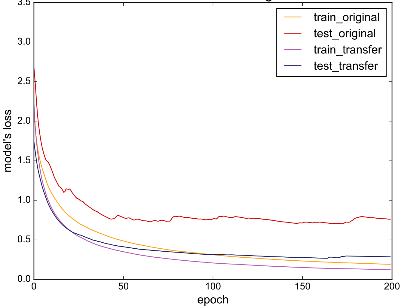
Source: ProximalPhalanxTW - Target: SwedishLeaf
