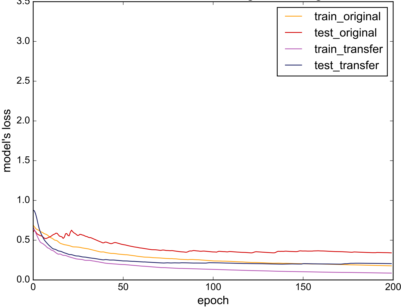
Source: ProximalPhalanxTW - Target: ToeSegmentation1
