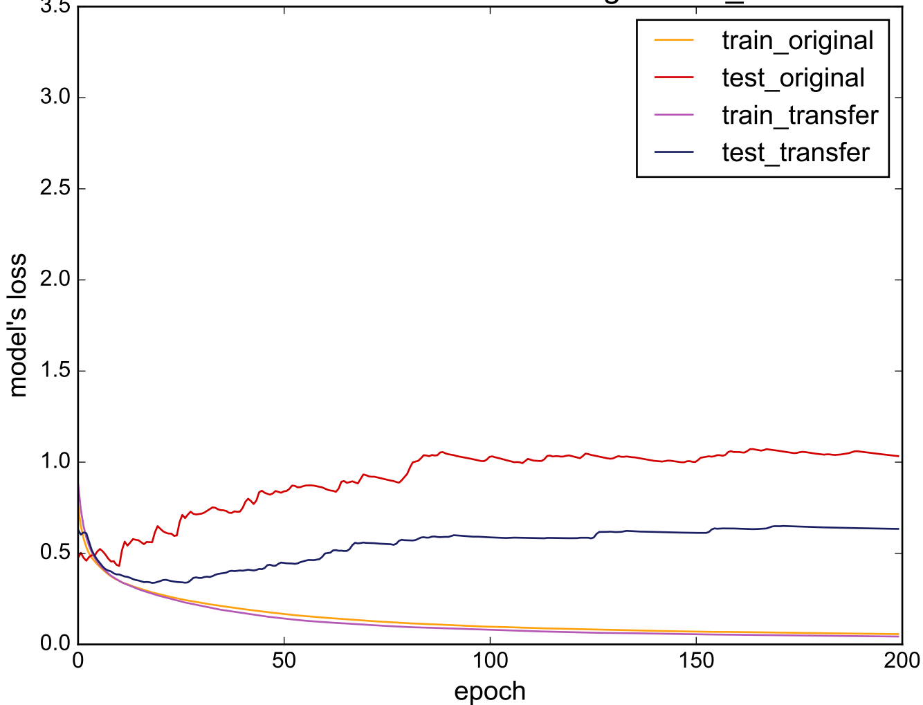
Source: ProximalPhalanxTW - Target: Two_Patterns
