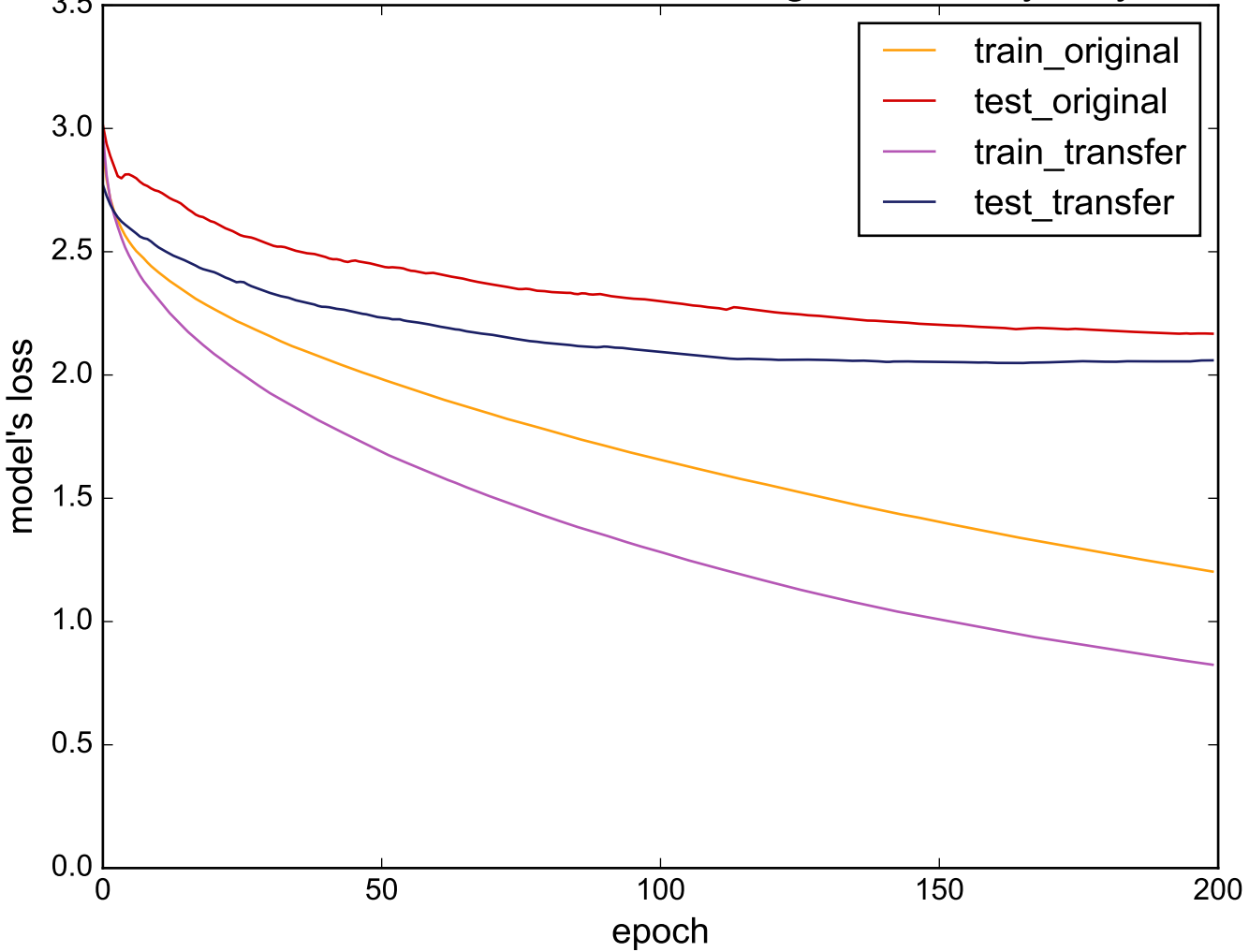
Source: ProximalPhalanxTW - Target: WordsSynonyms
