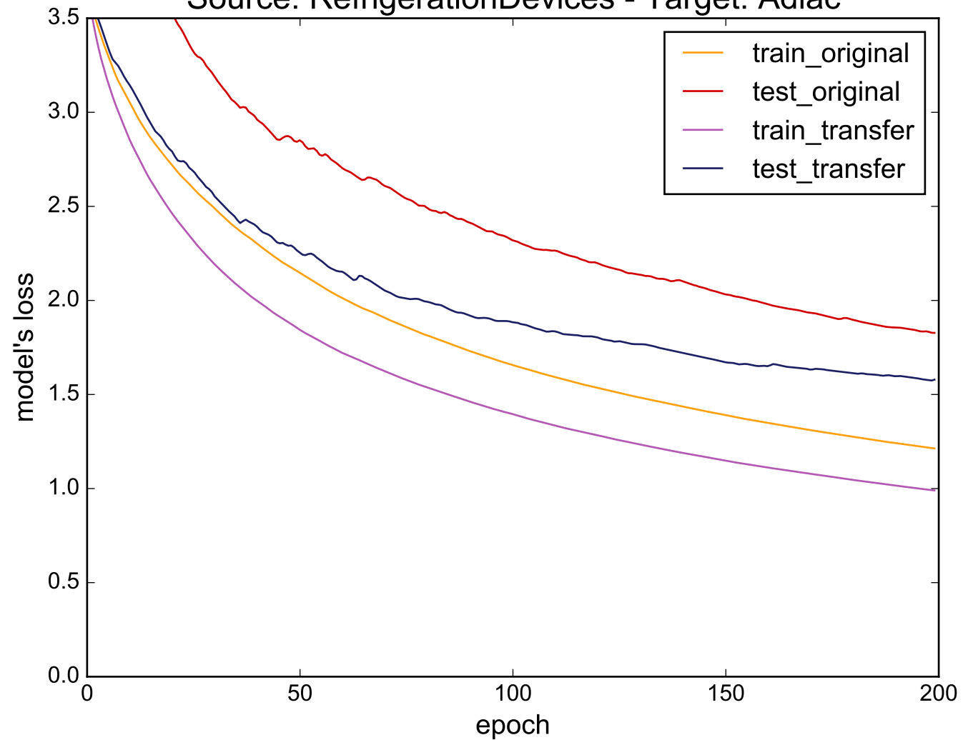
Source: RefrigerationDevices - Target: Adiac
