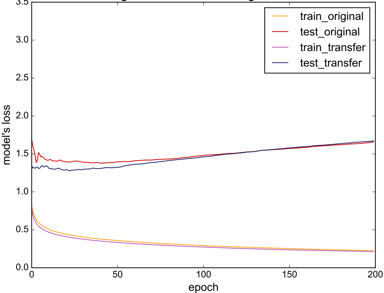
Source: RefrigerationDevices - Target: ElectricDevices
