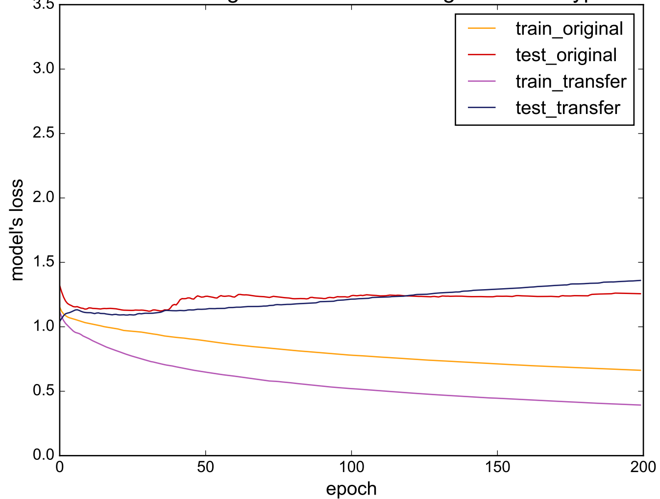
Source: RefrigerationDevices - Target: ScreenType
