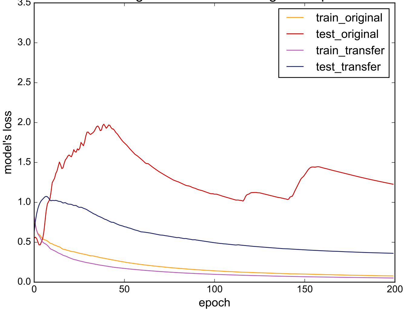
Source: RefrigerationDevices - Target: ShapeletSim
