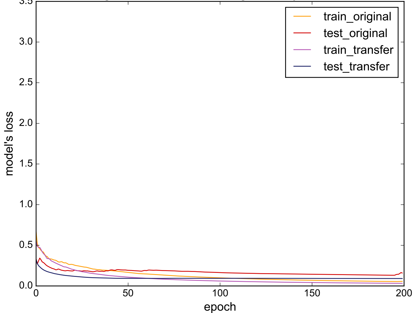
Source: RefrigerationDevices - Target: SonyAIBORobotSurface
