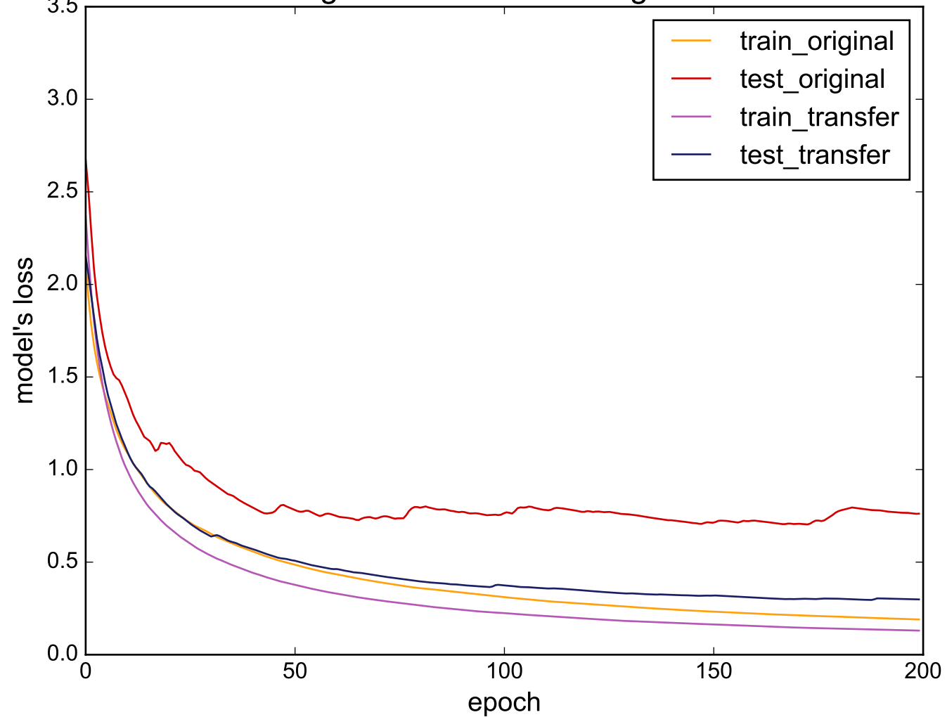
Source: RefrigerationDevices - Target: SwedishLeaf
