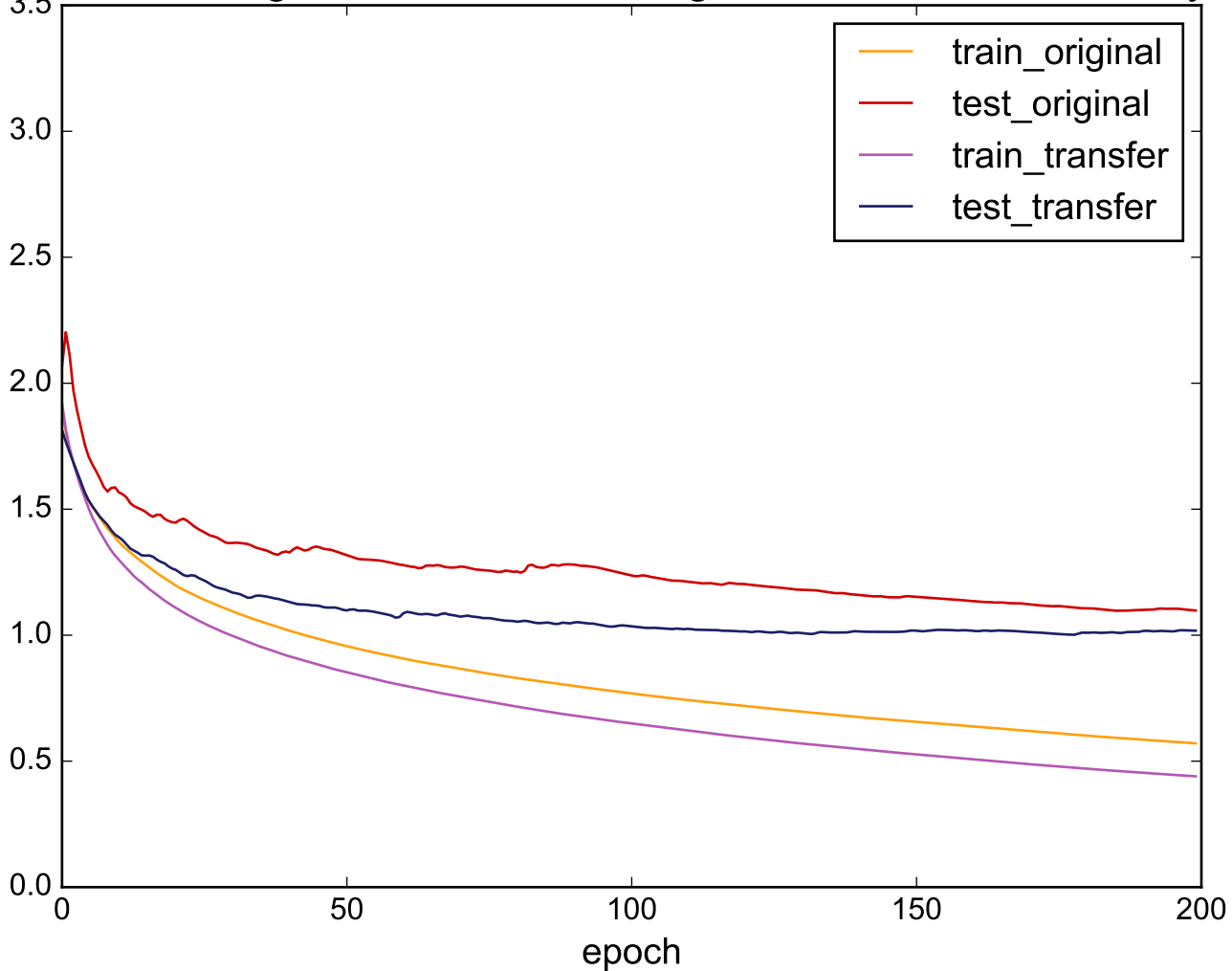
Source: RefrigerationDevices - Target: UWaveGestureLibraryAll
