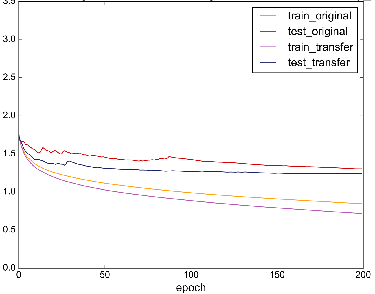
Source: RefrigerationDevices - Target: uWaveGestureLibrary_Y
