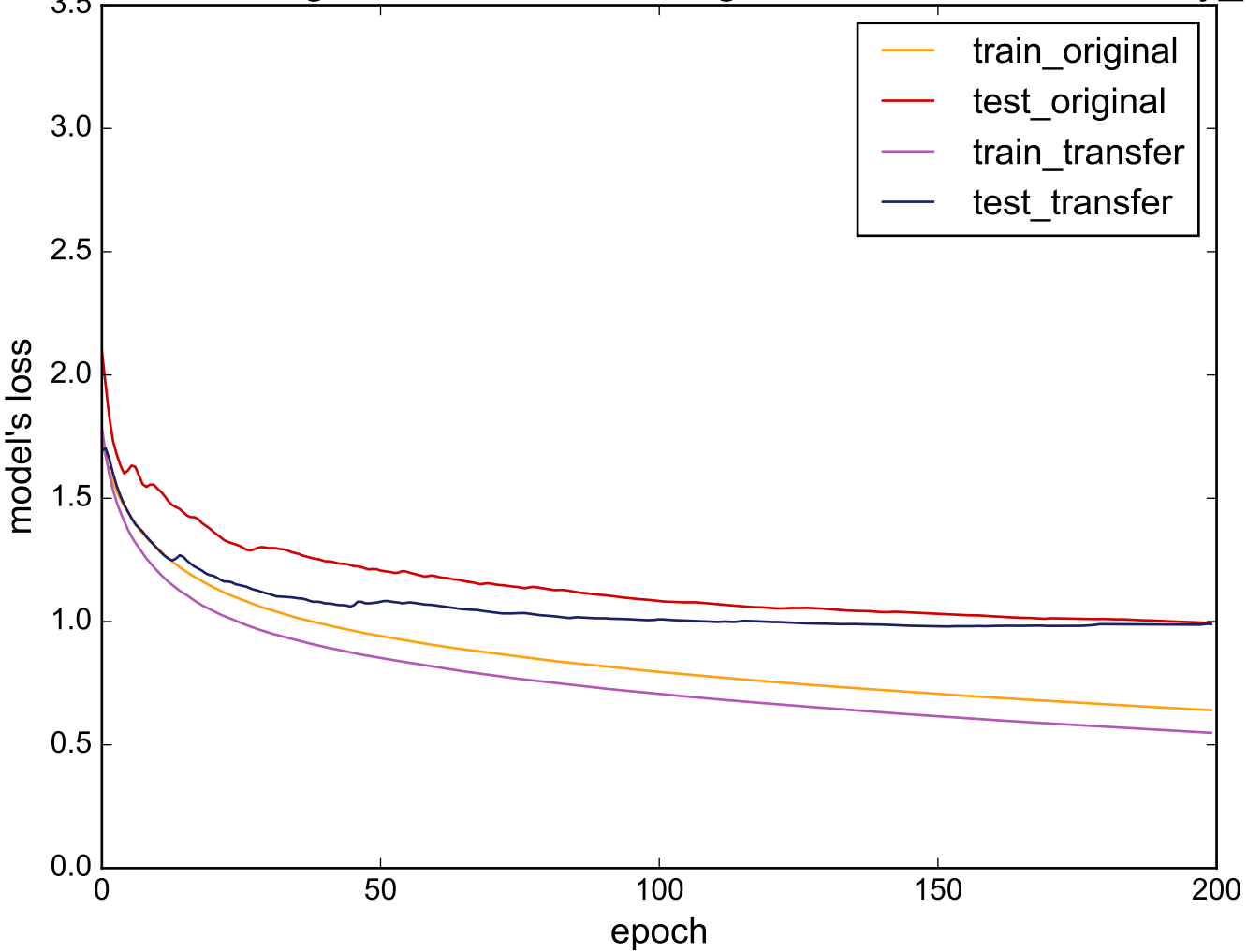
Source: RefrigerationDevices - Target: uWaveGestureLibrary_Z
