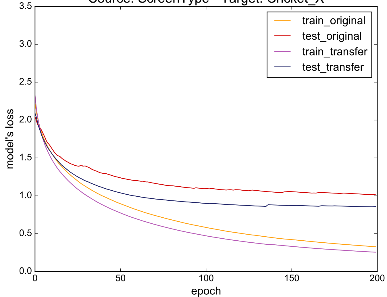
Source: ScreenType - Target: Cricket_X
