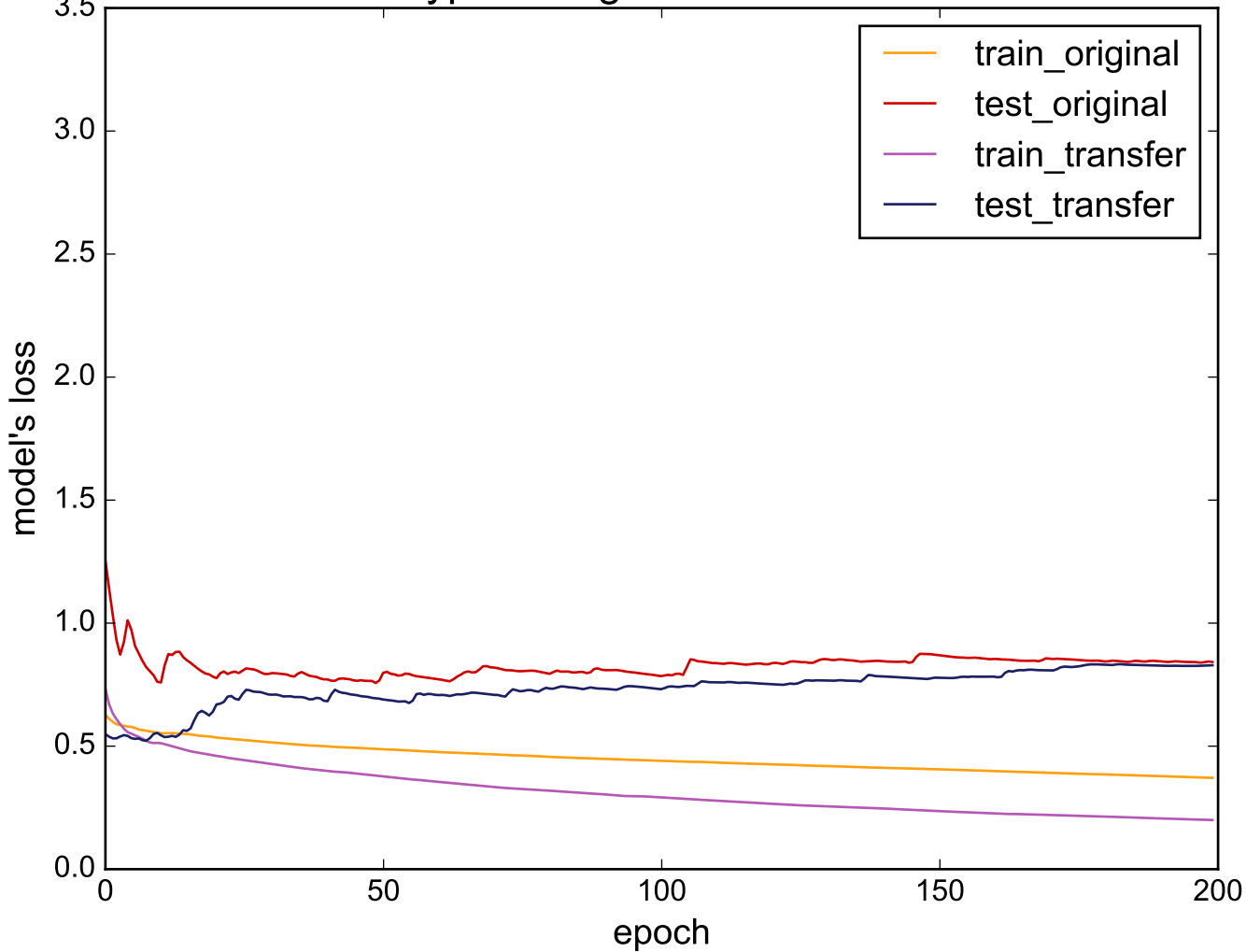
Source: ScreenType - Target: DistalPhalanxOutlineCorrect
