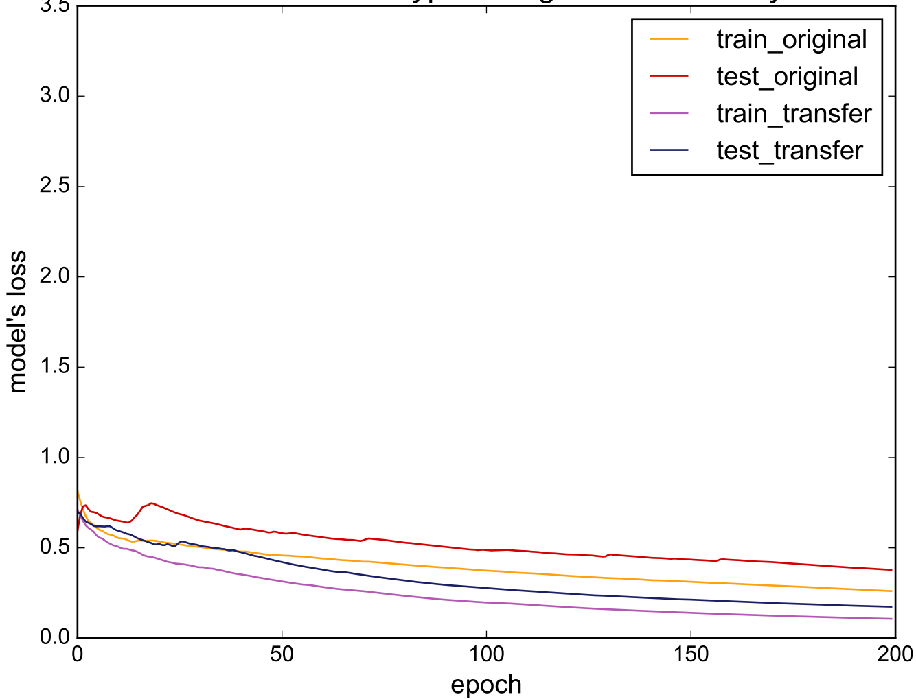
Source: ScreenType - Target: ECGFiveDays
