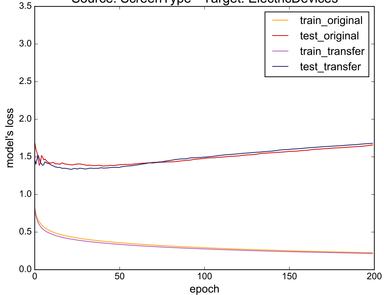
Source: ScreenType - Target: ElectricDevices
