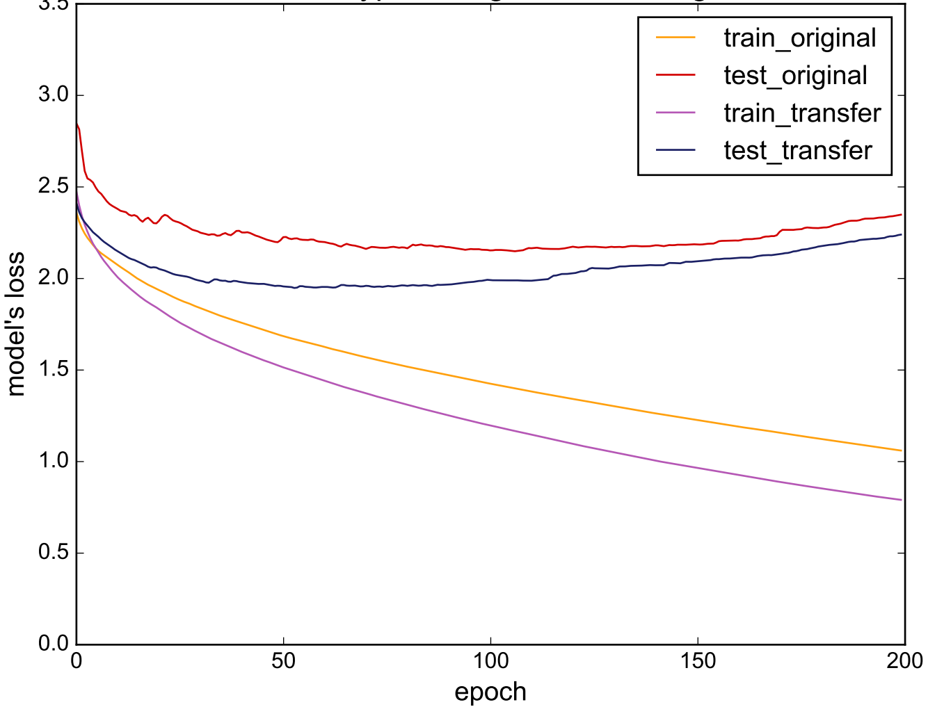
Source: ScreenType - Target: InsectWingbeatSound
