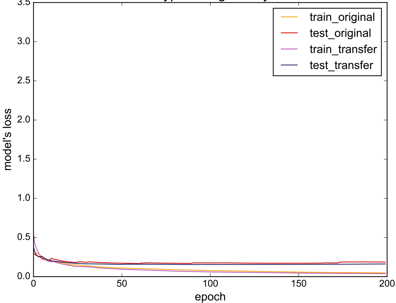
Source: ScreenType - Target: ItalyPowerDemand
