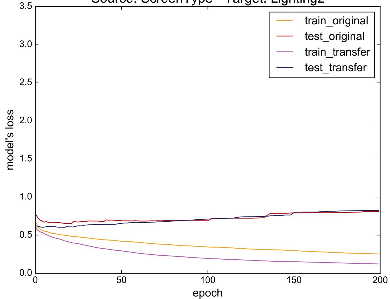
Source: ScreenType - Target: Lighting2
