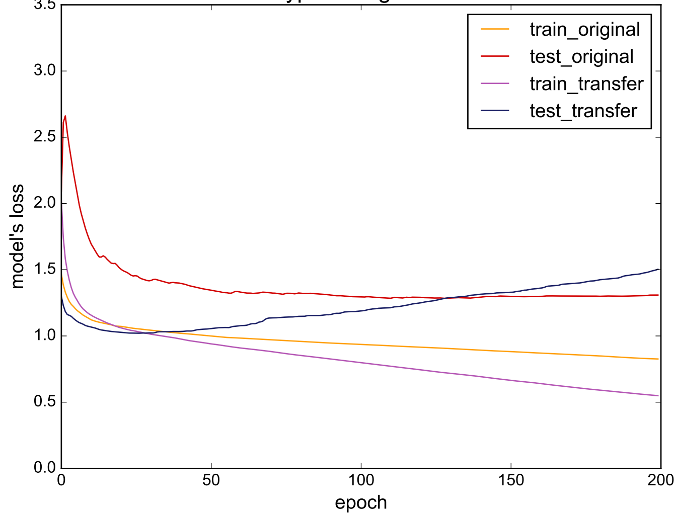
Source: ScreenType - Target: MiddlePhalanxTW
