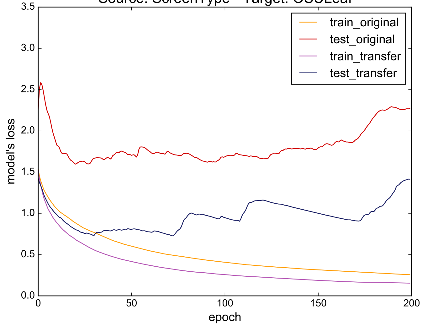
Source: ScreenType - Target: OSULeaf
