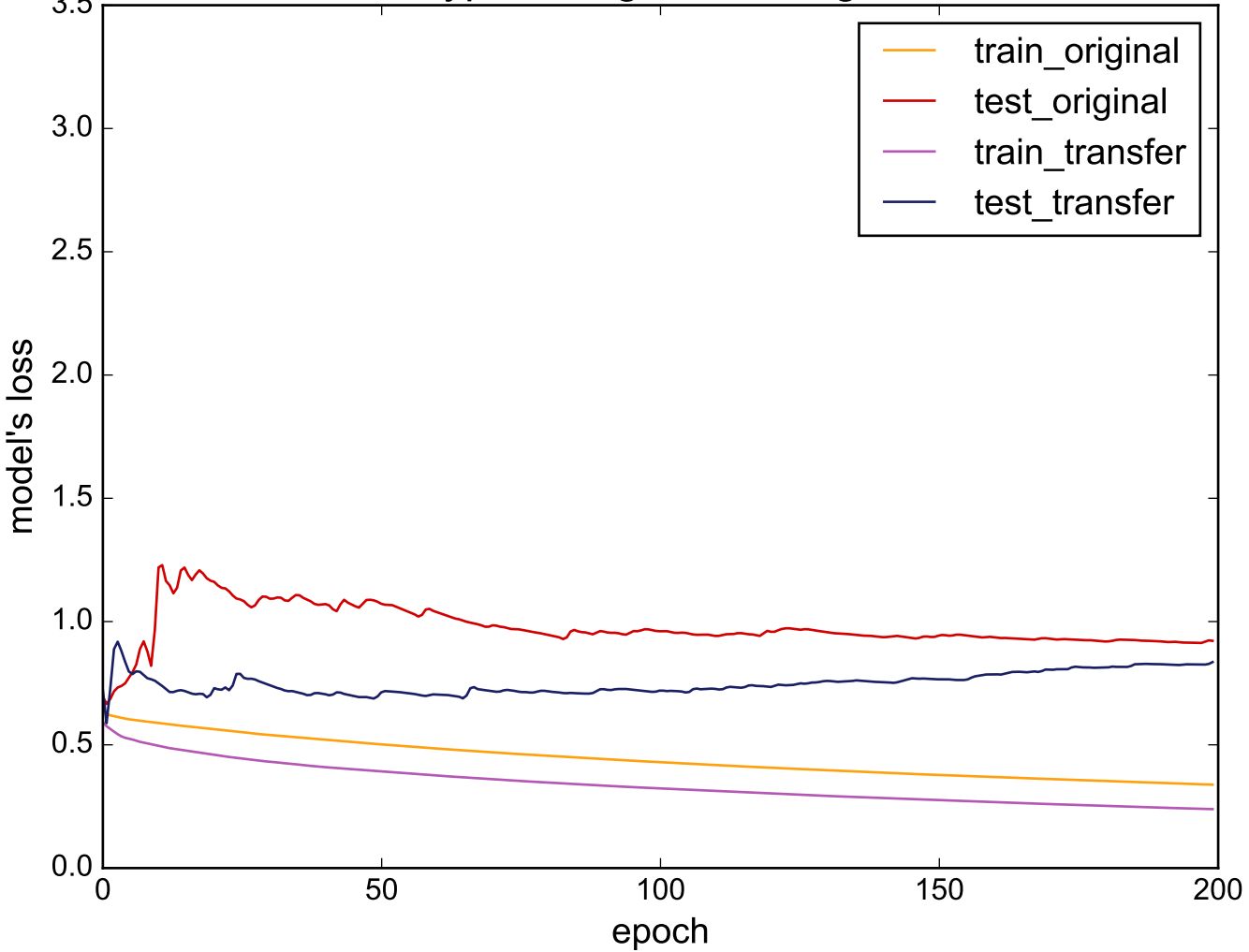
Source: ScreenType - Target: PhalangesOutlinesCorrect
