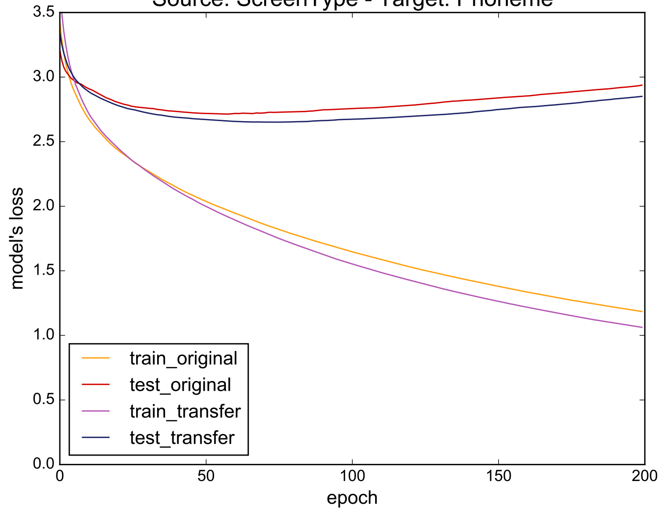
Source: ScreenType - Target: Phoneme
