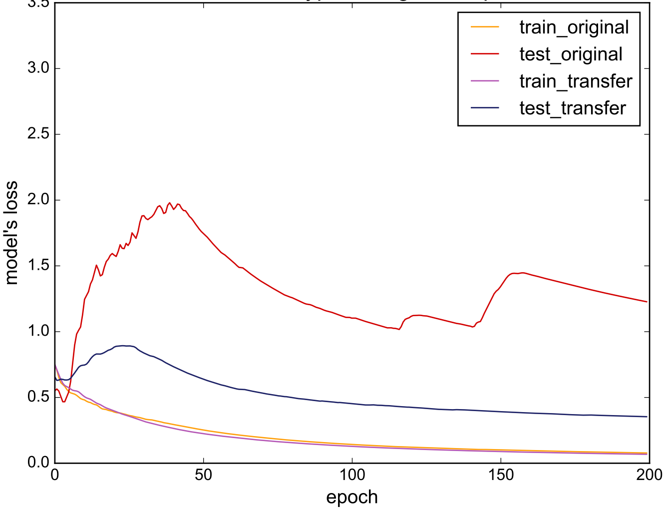
Source: ScreenType - Target: ShapeletSim
