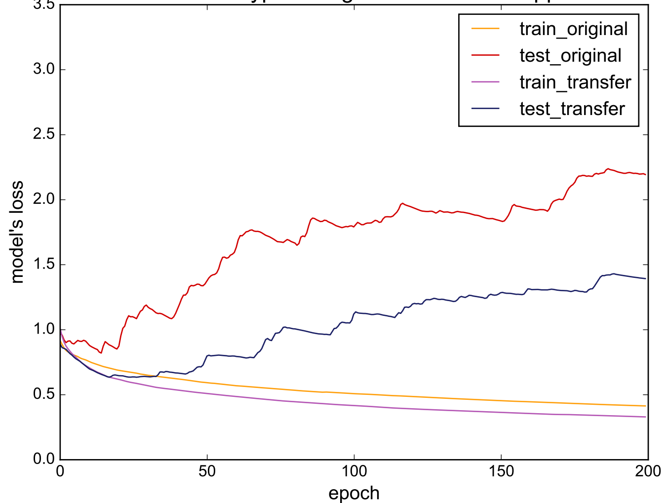
Source: ScreenType - Target: SmallKitchenAppliances
