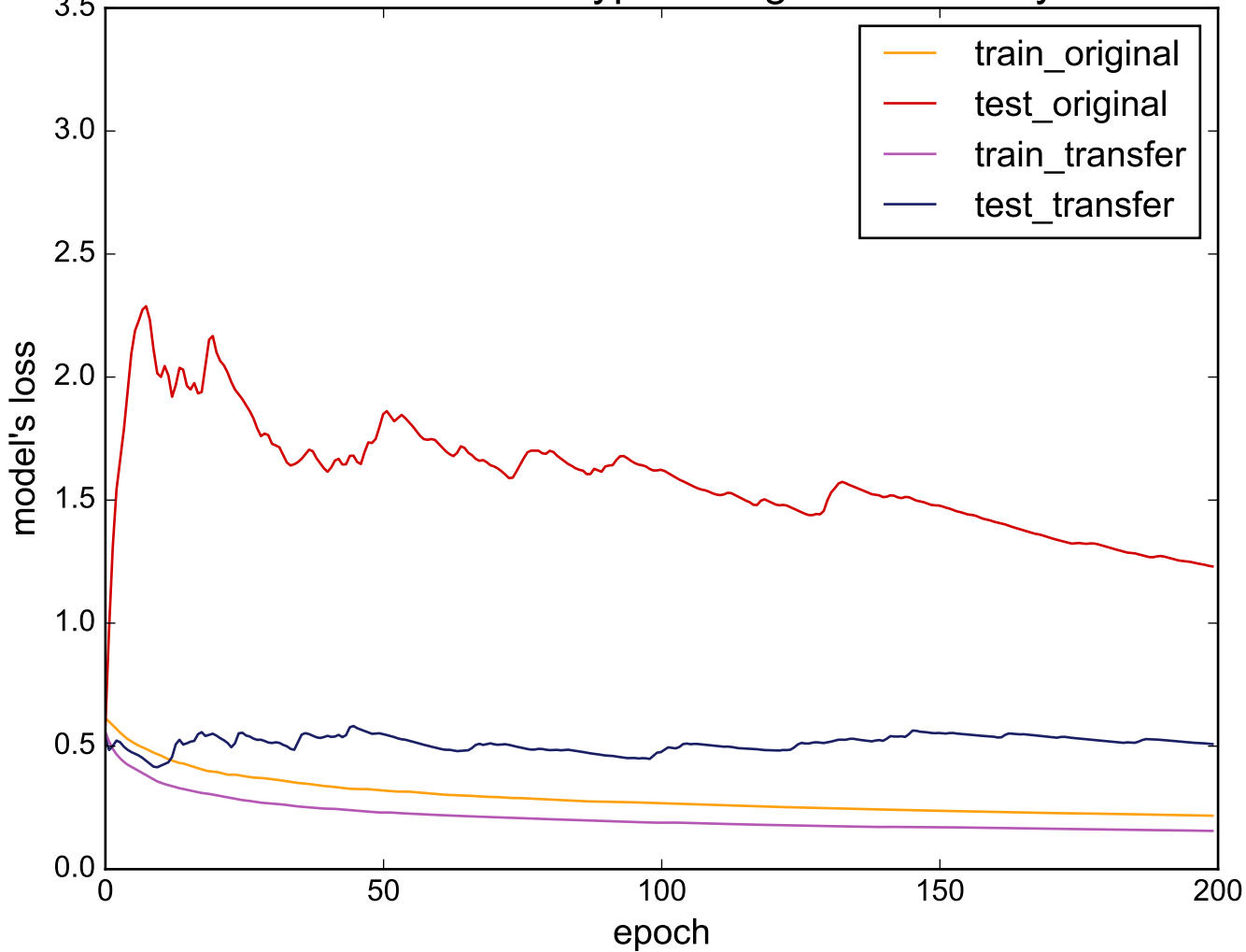
Source: ScreenType - Target: Strawberry
