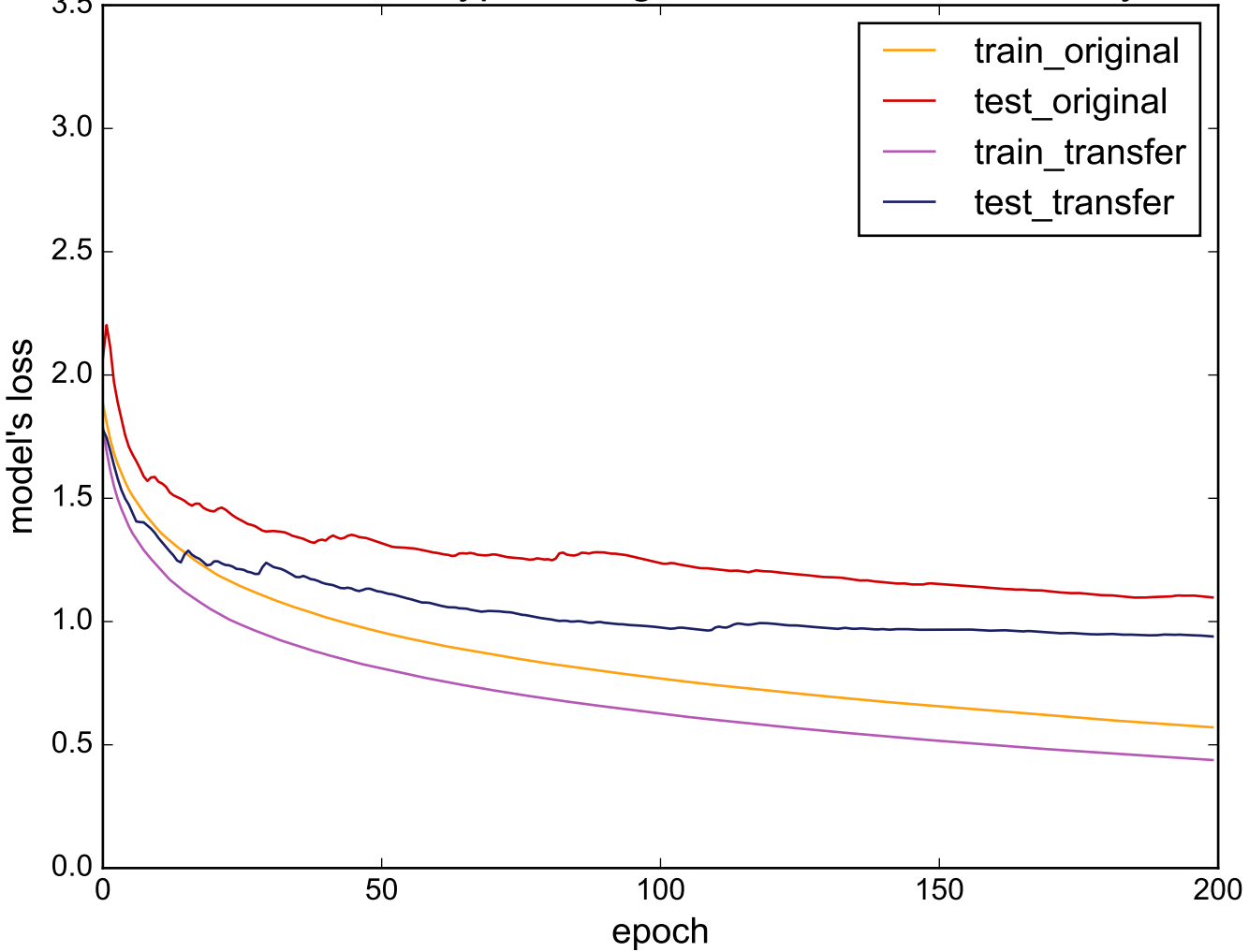
Source: ScreenType - Target: UWaveGestureLibraryAll
