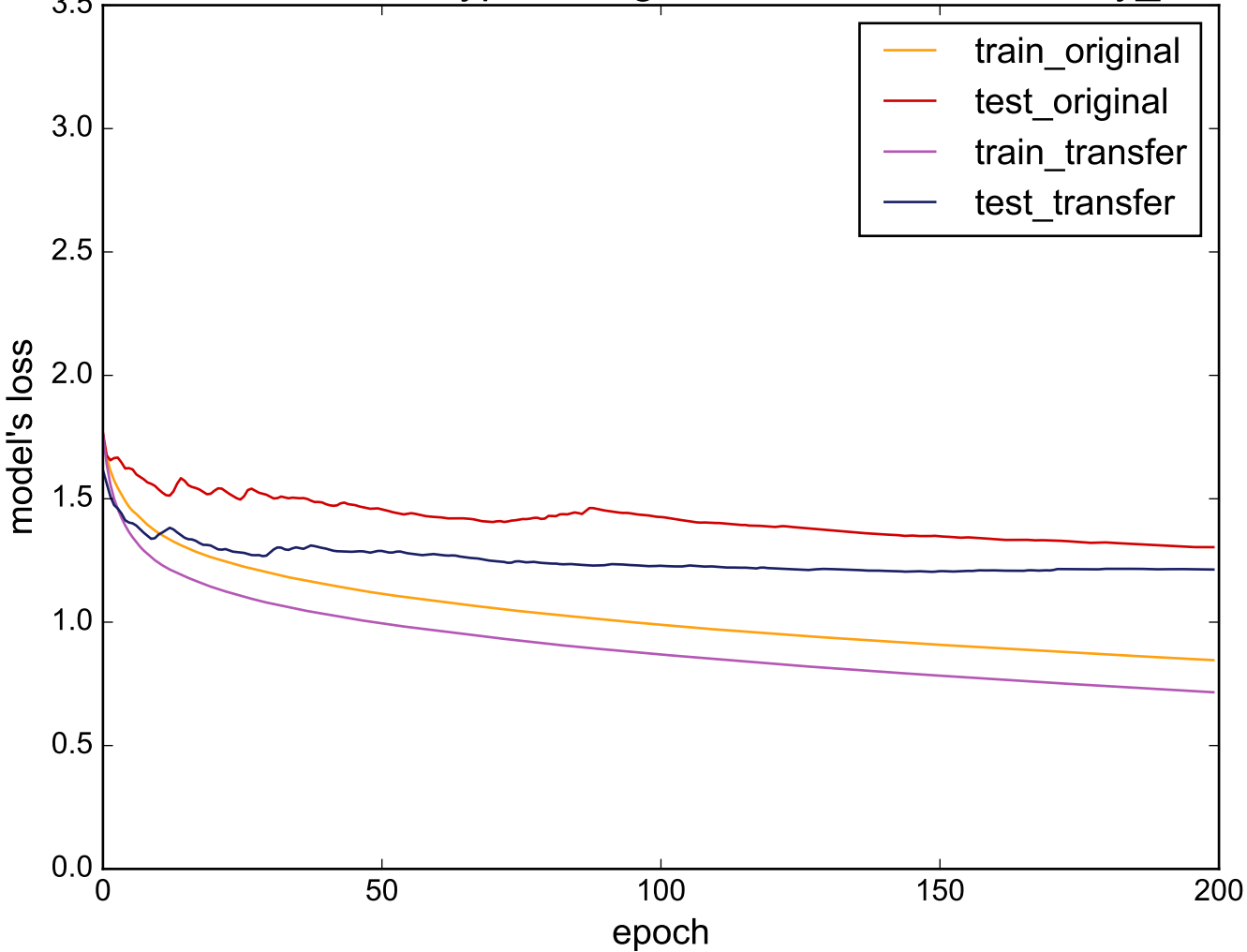
Source: ScreenType - Target: uWaveGestureLibrary_Y
