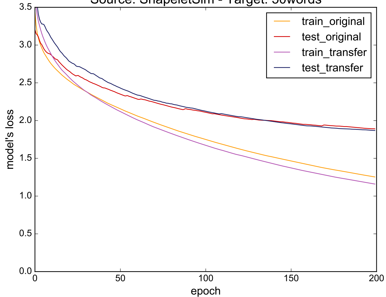
Source: ShapeletSim - Target: 50words
