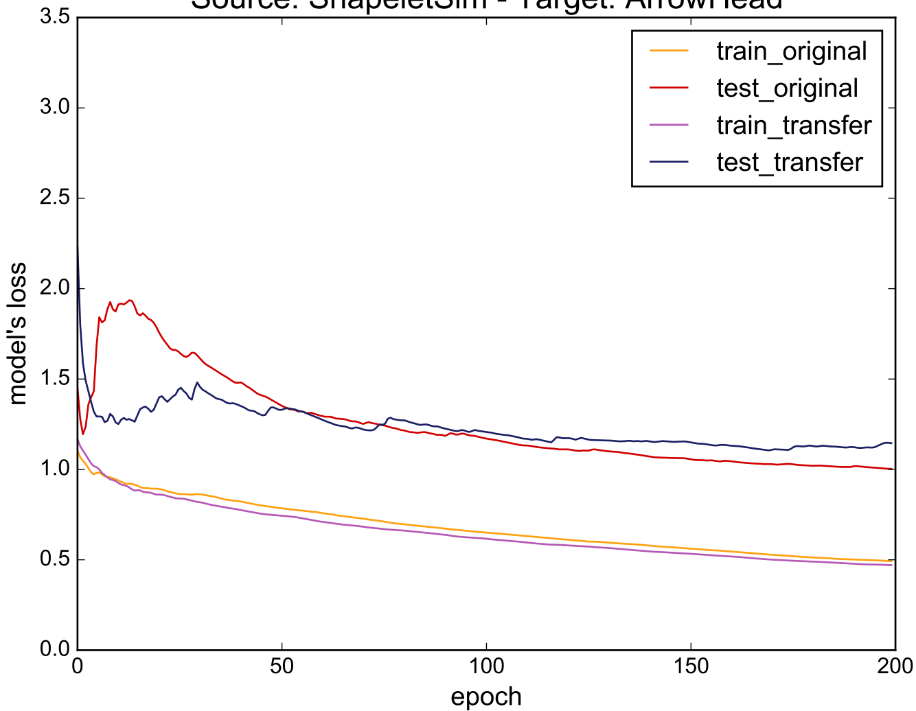
Source: ShapeletSim - Target: ArrowHead
