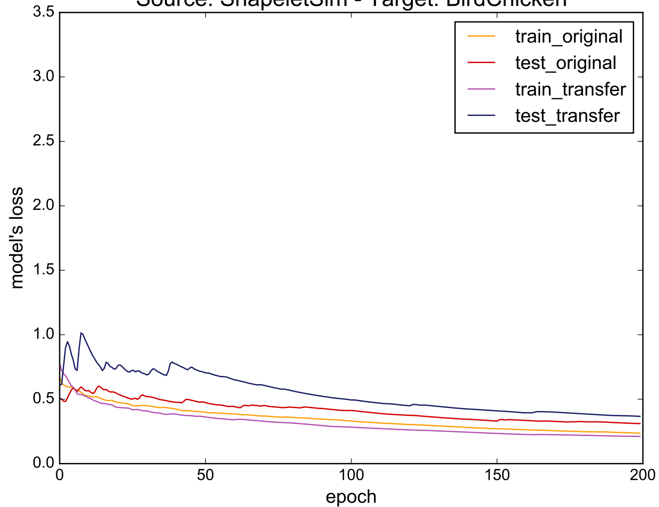
Source: ShapeletSim - Target: BirdChicken
