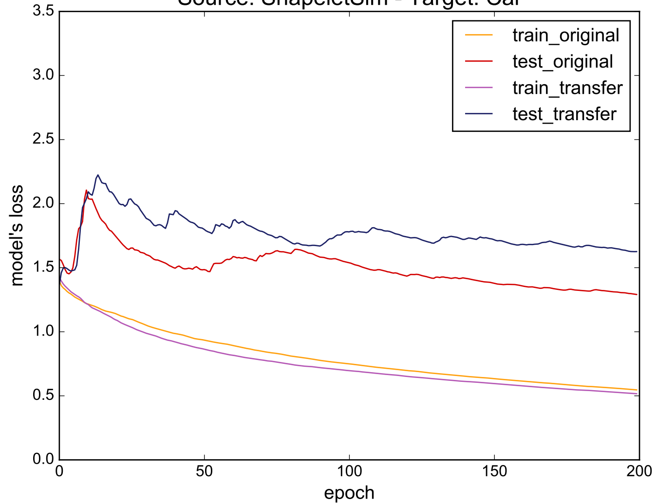
Source: ShapeletSim - Target: Car
