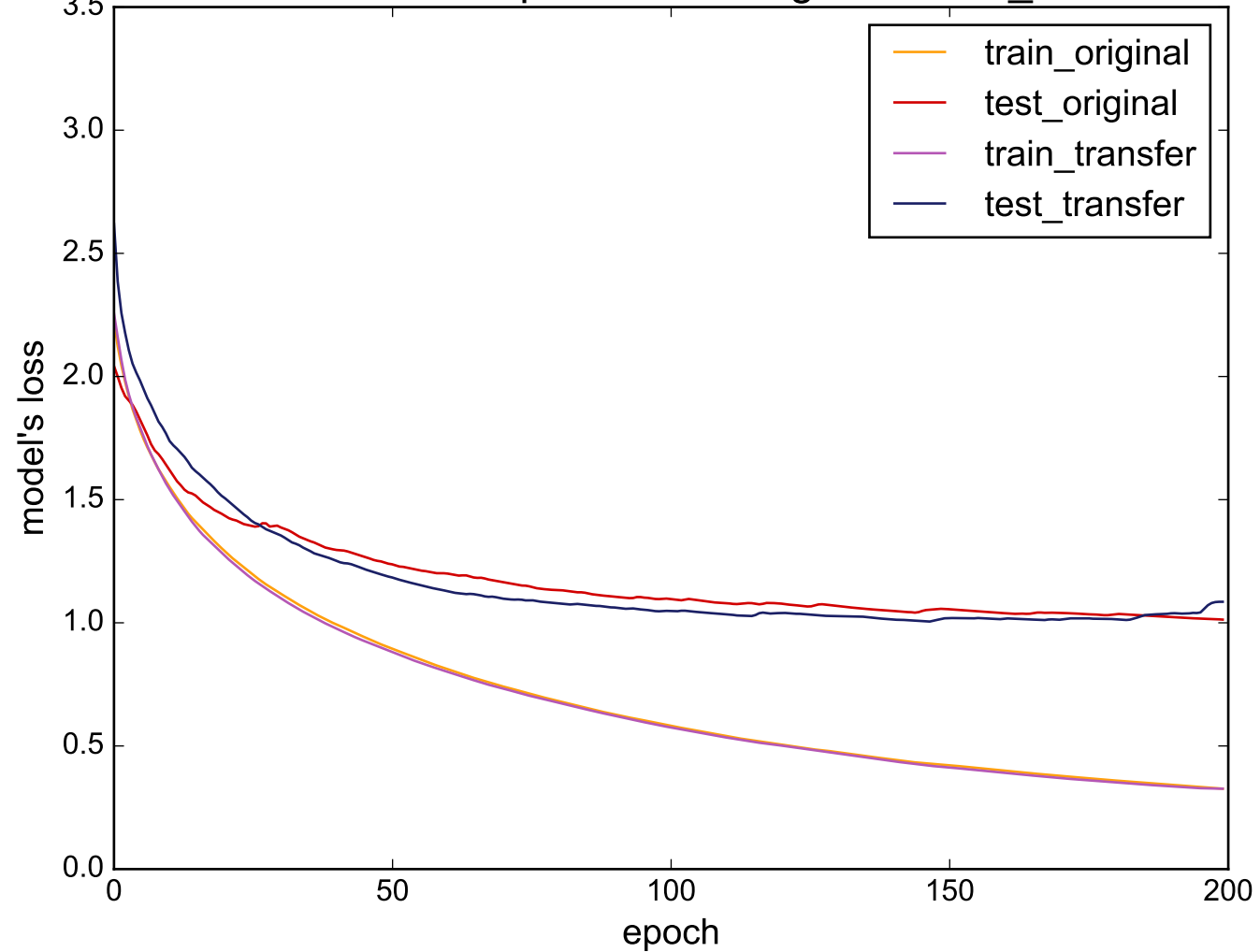
Source: ShapeletSim - Target: Cricket_X
