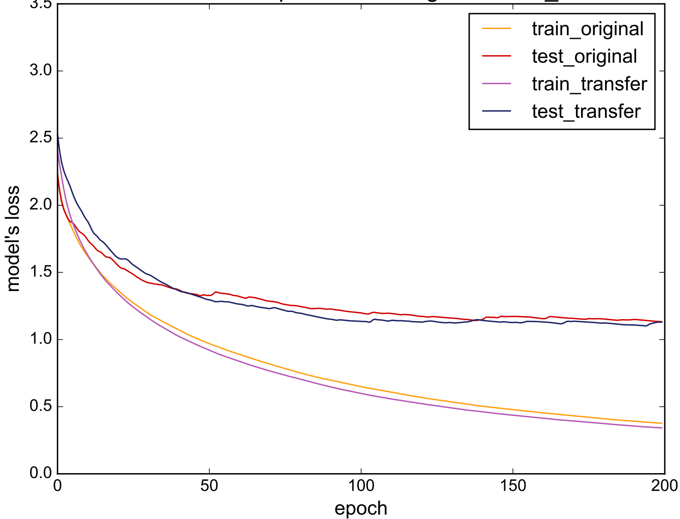
Source: ShapeletSim - Target: Cricket_Y
