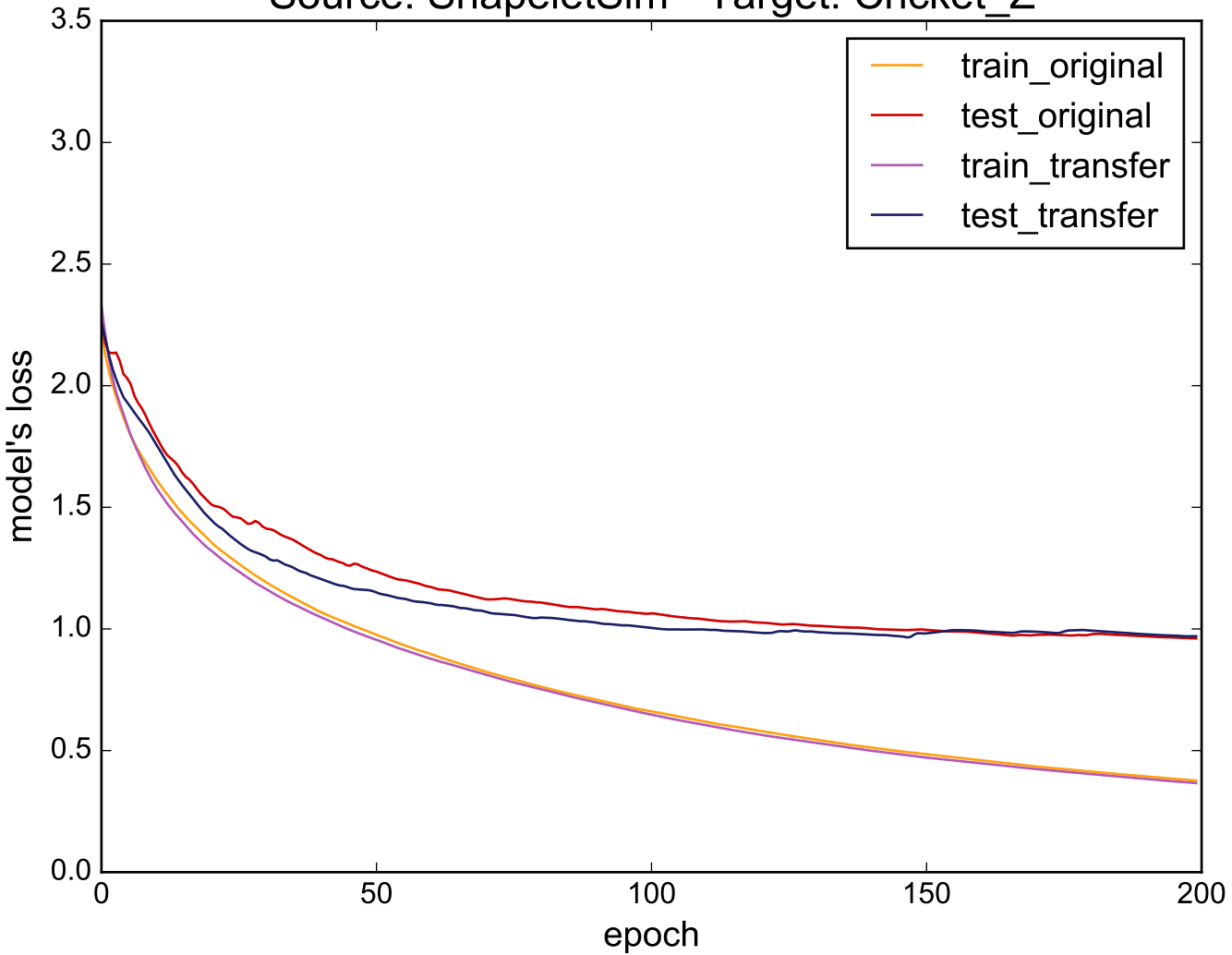
Source: ShapeletSim - Target: Cricket_Z
