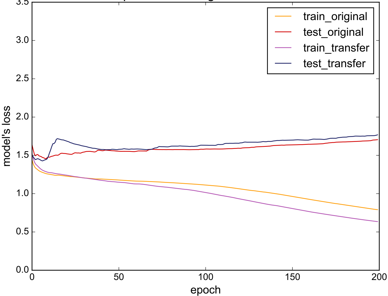
Source: ShapeletSim - Target: DiatomSizeReduction
