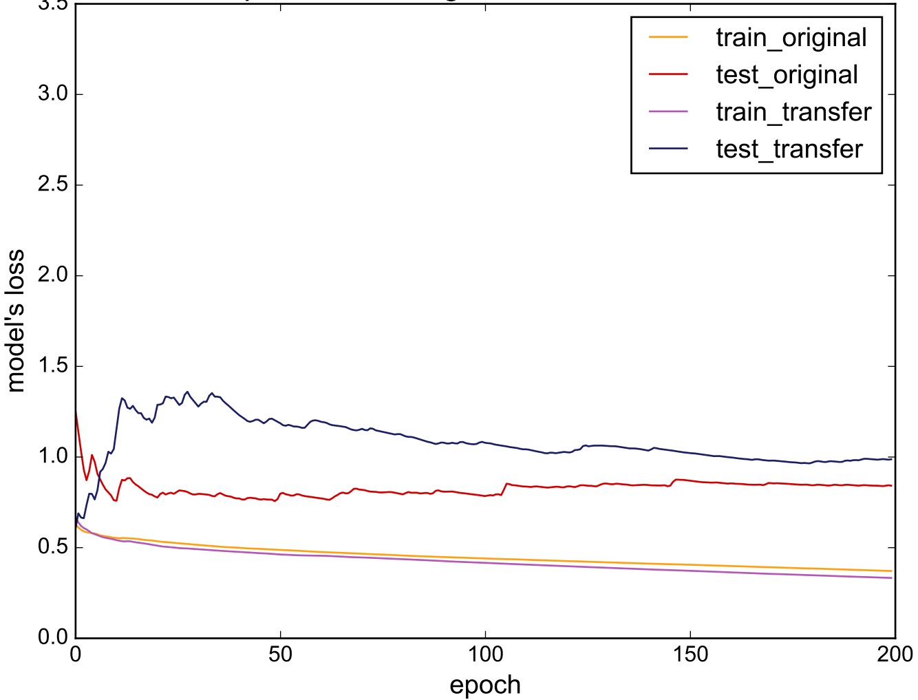
Source: ShapeletSim - Target: DistalPhalanxOutlineCorrect
