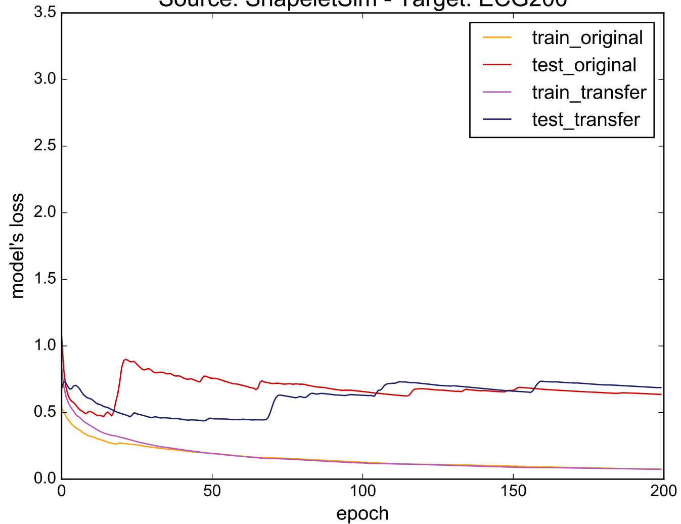
Source: ShapeletSim - Target: ECG200
