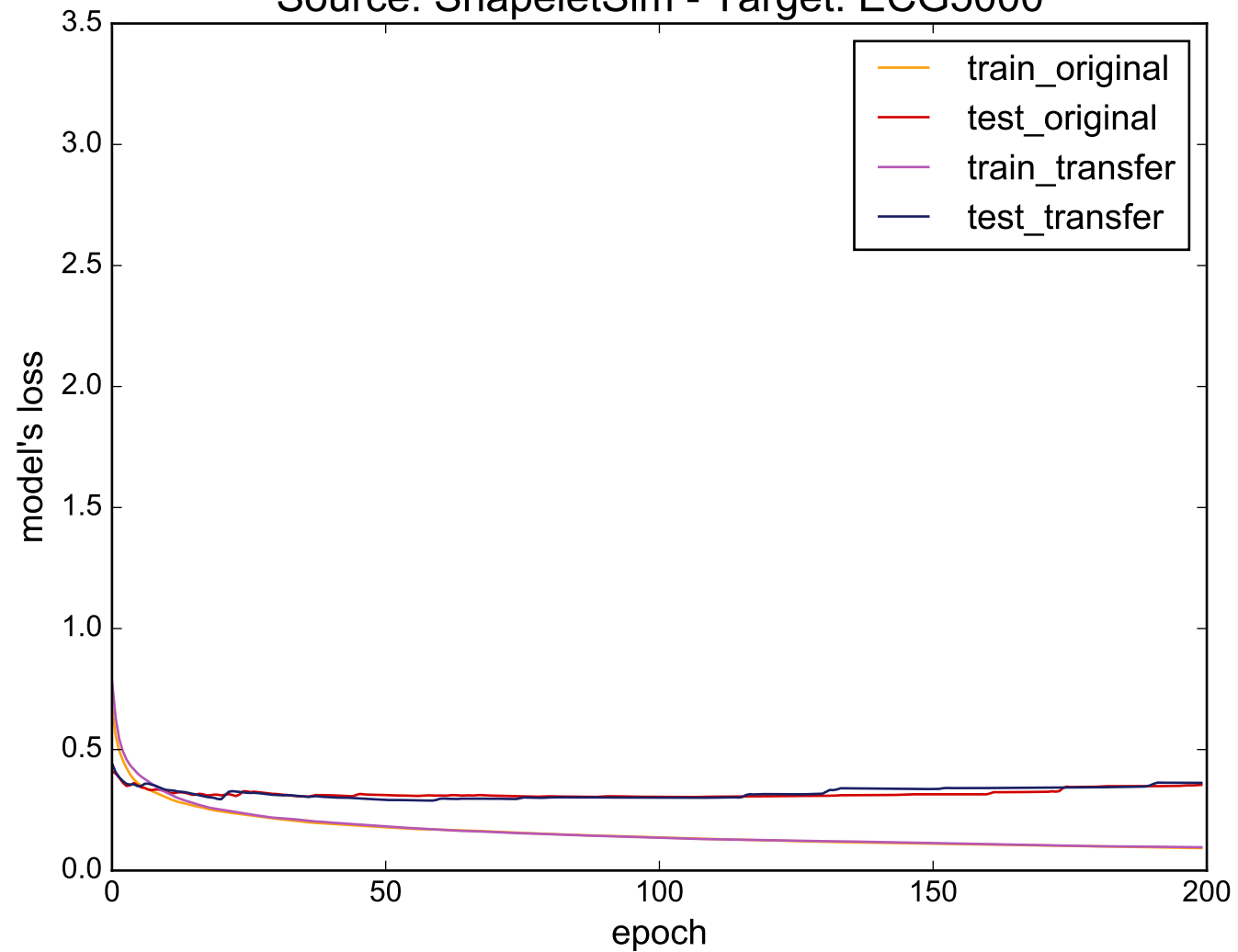
Source: ShapeletSim - Target: ECG5000
