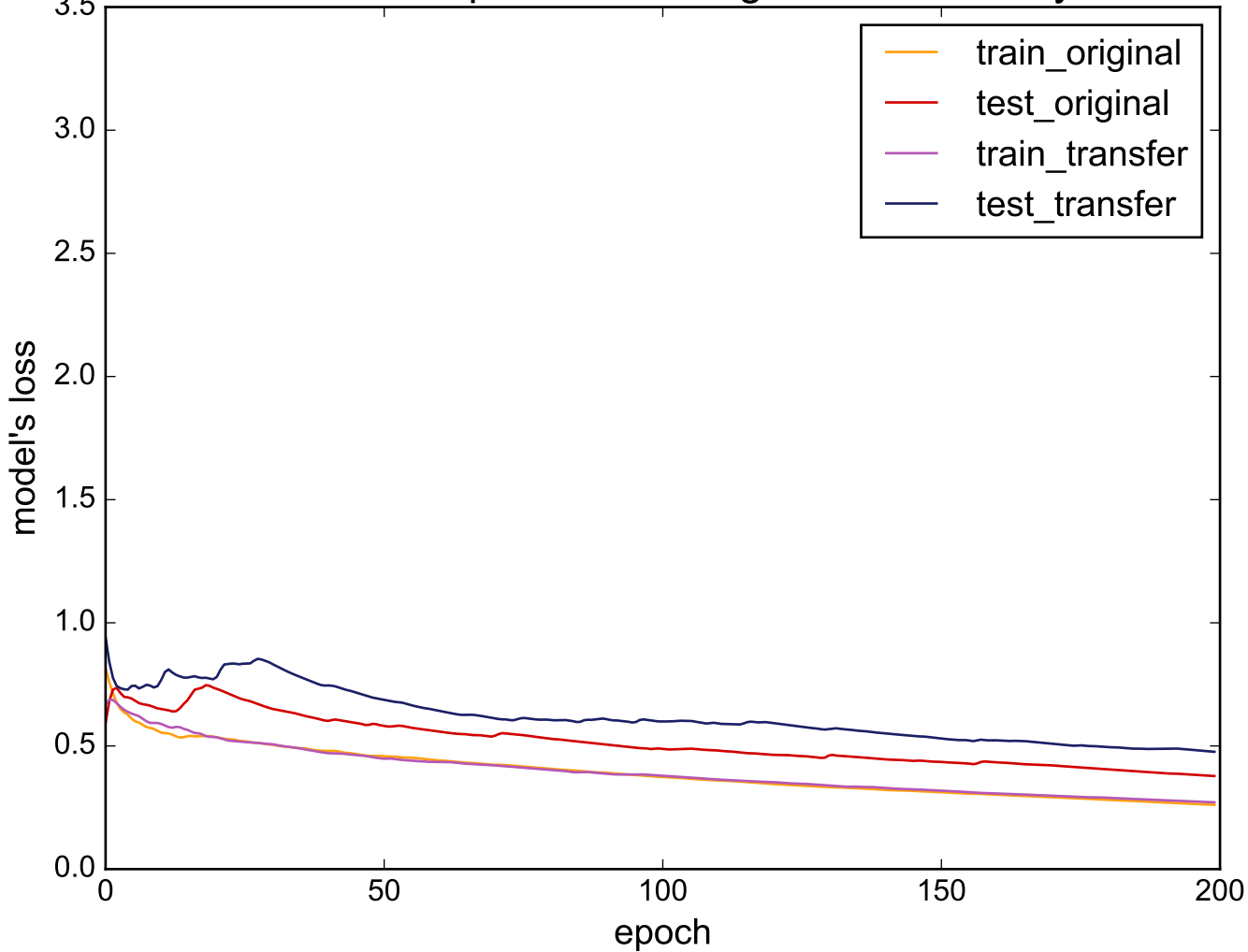
Source: ShapeletSim - Target: ECGFiveDays
